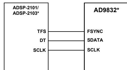
Figure 28. ADSP-2101/ADSP-2103 to AD9832 Interface
