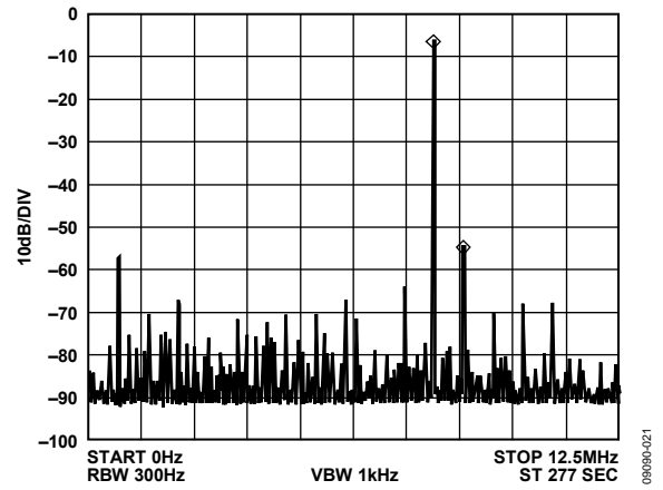
Figure 21. f_{CLK} = 25 MHz, f_{OUT} = 8.1 MHz, Frequency Word = 0x52F1A9FC
