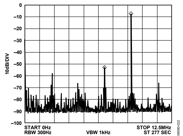
Figure 22. f_{CLK} = 25 MHz, f_{OUT} = 9.1 MHz, Frequency Word = 0x5D2F1AA0
