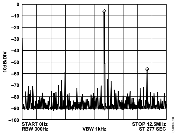
Figure 20. f_{CLK} = 25 MHz, f_{OUT} = 7.1 MHz, Frequency Word = 0x48B43958
