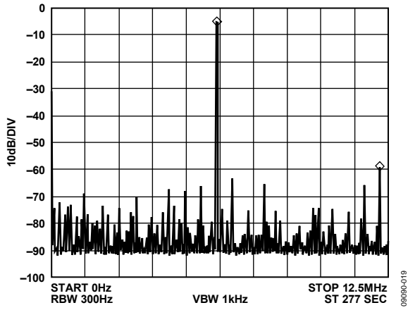
Figure 19. f_{CLK} = 25 MHz, f_{OUT} = 6.1 MHz, Frequency Word = 0x3E76C8B4
